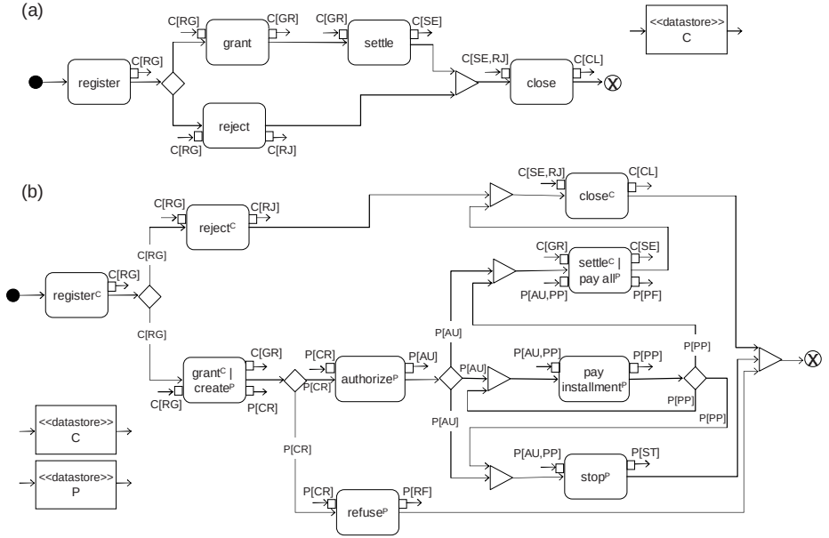
Fig. 8. Generated process models: (a) from Claim object life cycle (b) from both Claim and Payment object life cycles
