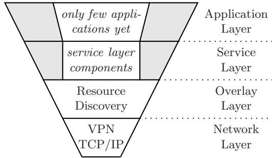
Fig. 1. Layers for Peer-to-Peer Based Applications
